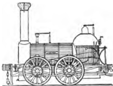
Fig. 96. —Bury's first Inside-cylinder Engine, "Liverpool," completed March, 1831; sent to America.
